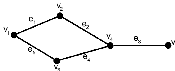
Figure 3.12: Illustrating Planar Straight Line Graph (PSLG)
