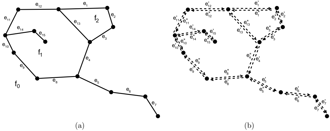
Figure 3.5: Gabriel graph showing edges and its equivalent half edge
