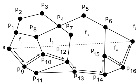
Figure 2.8: Illustrating Face Routing
